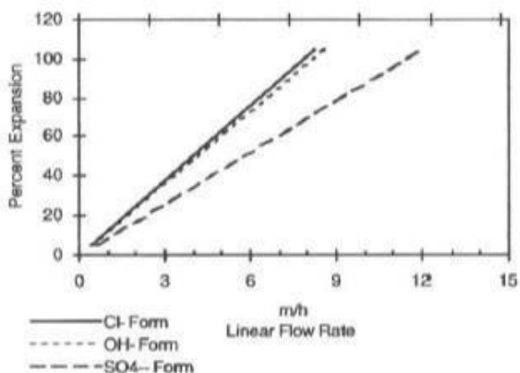
Figure 1. Bed expansion
