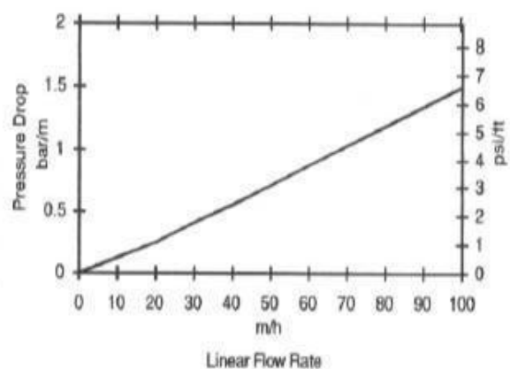
Figure 2. Pressure Drop
