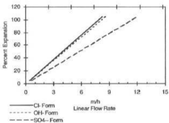
Figure 1. Bed expansion
